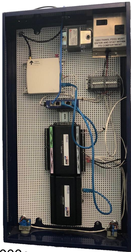
JENE-3000e
